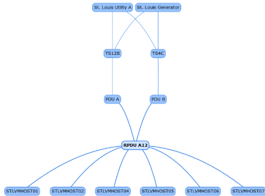
Visual view of power chain
