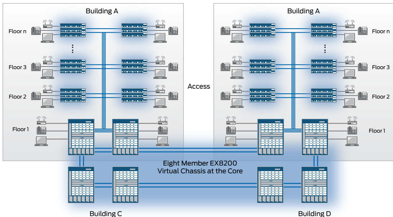
Figure 2: A campus aggregation/core environment can be managed as a single device with an EX8208 Virtual Chassis configuration.
