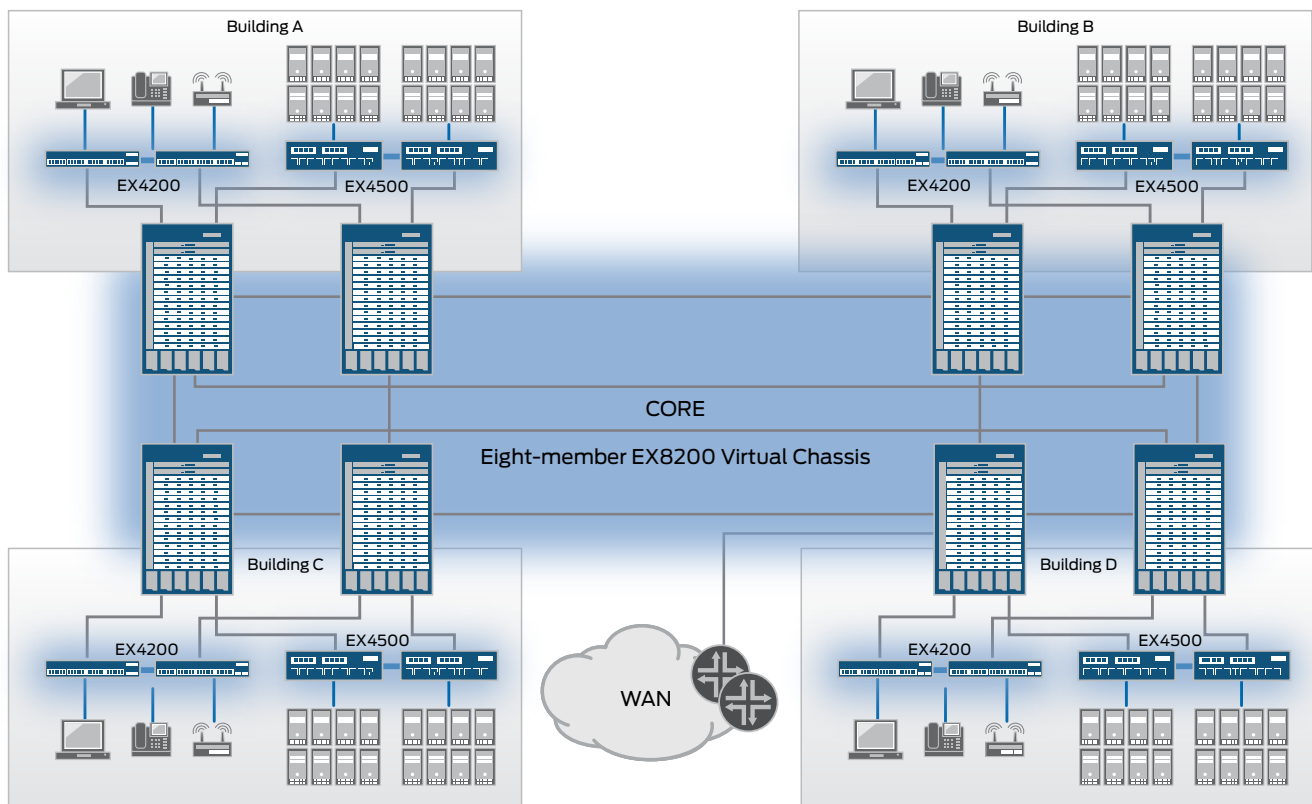
Figure 1: Eight-member EX8216 Virtual Chassis configuration in the core, managed as a single, logical switch.
